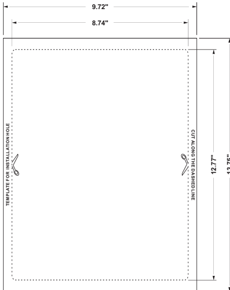
Dimensions for ceiling cutting
